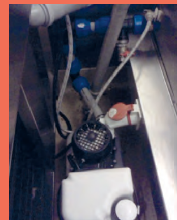
Instalace SANICOM®
