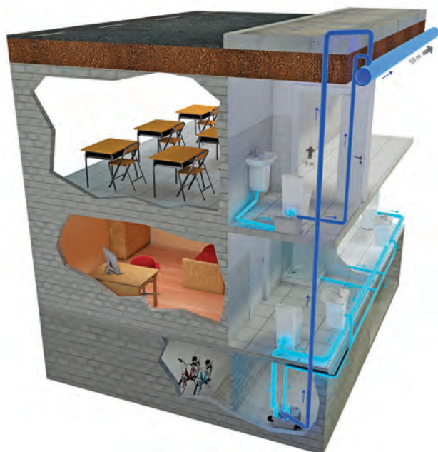
SANICUBIC® 2 Classic
